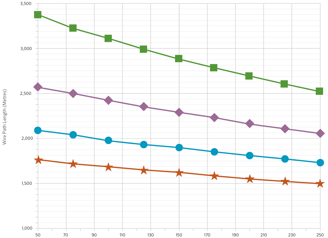
Active Stations Based on Wire Length and Number of Two-Way Modules Using ID1 (2.2 mm 2 ) Wire
